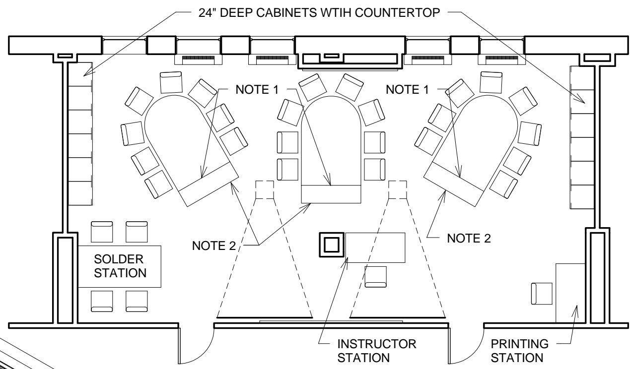
1 OPTION 1 1/8" = 1'-0"
